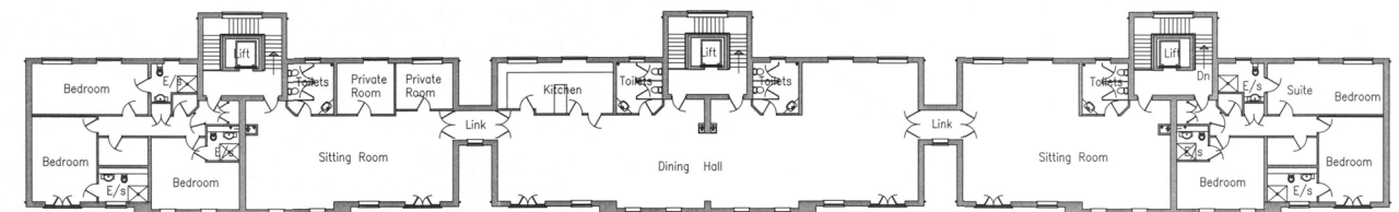
Fourth Floor Plan
